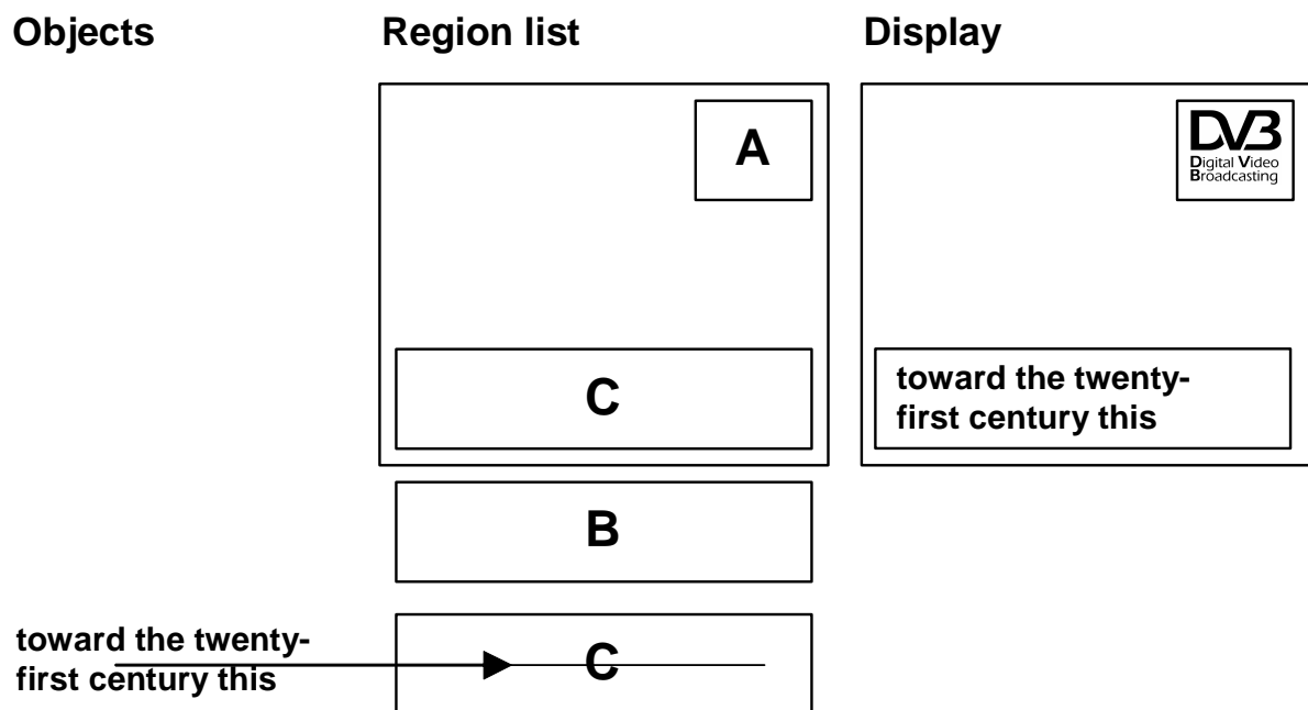
Figure A.4: Deliver then reveal second text
