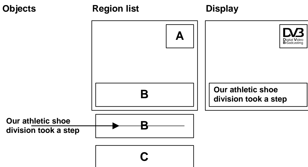
Figure A.3: Deliver then reveal first text
